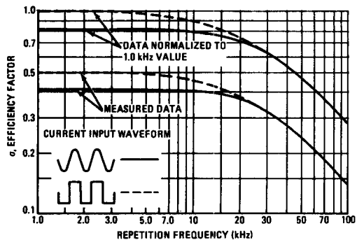
FIGURE 15 – RECTIFICATION WAVEFORM EFFICIENCY
