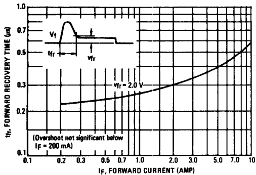
FIGURE 13 – FORWARD RECOVERY TIME
