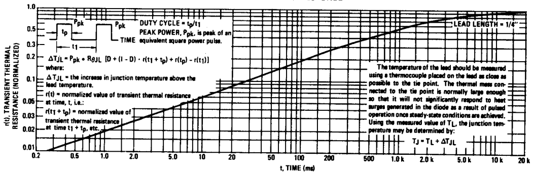
FIGURE 10 – THERMAL RESPONSE
