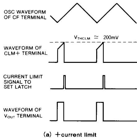
(a) +current limit
