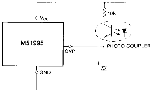
Fig. 28 Peripheral circuit of OVP terminal
