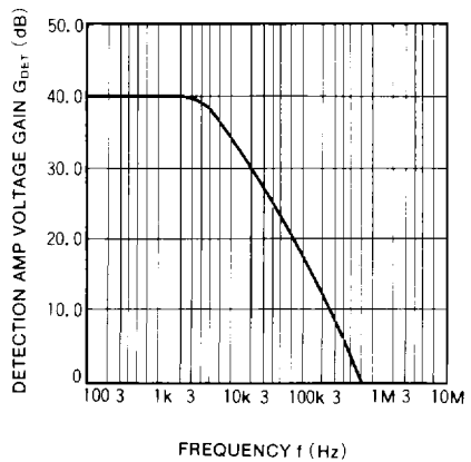
DETECTION AMP VOLTAGE GAIN VS. FREQUENCY
