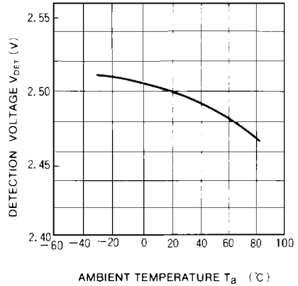
DETECTION VOLTAGE VS. AMBIENT TEMPERATURE
