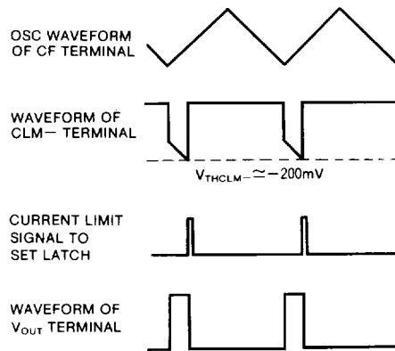
(b) -current limit
