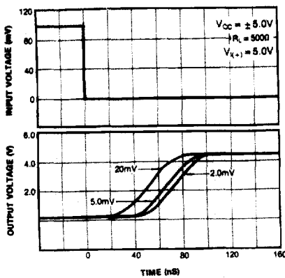
Fig. 5 RESPONSE TIME FOR VARIOUS INPUT OVERDRIVE
