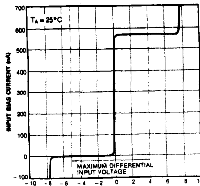
Fig. 6 INPUT CHARACTERISTICS
