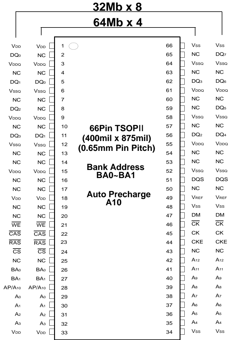
256Mb TSOPII Package Pinout
