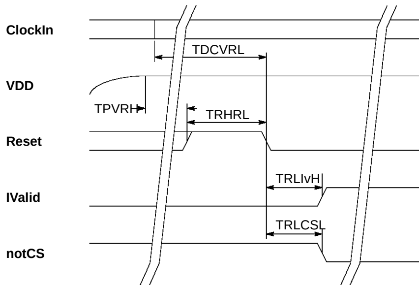
Figure 3.3 Reset timing
