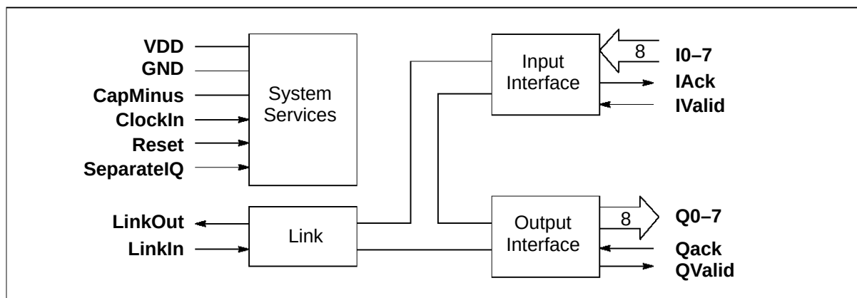
Figure 1.1 IMS C011 Mode 1 block diagram
