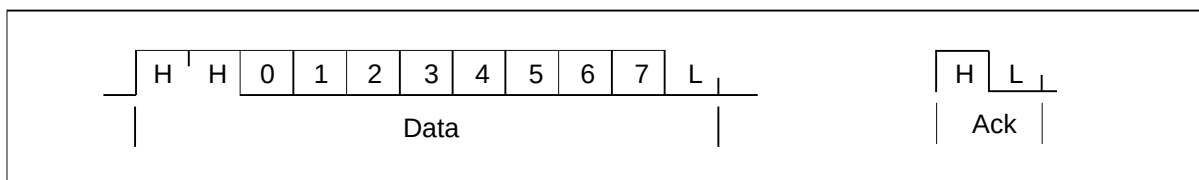
Figure 4.1 IMS C011 link data and acknowledge packets
