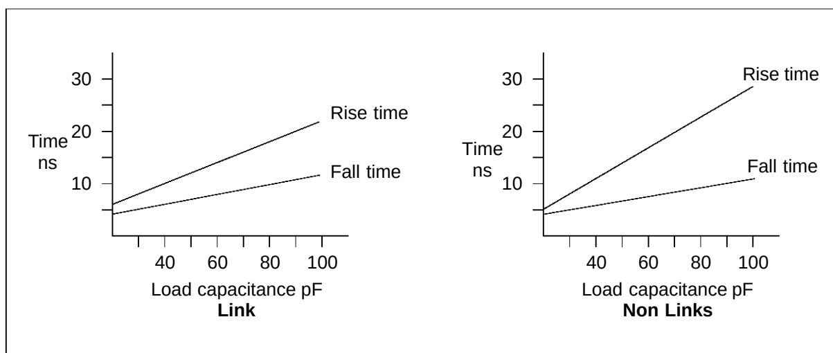
Figure 7.5 Typical rise/fall times
