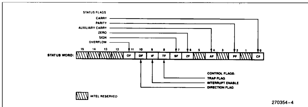
Figure 3b. Status Word Format 1-67
