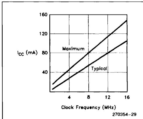
Figure 46. I_{CC} vs Frequency
