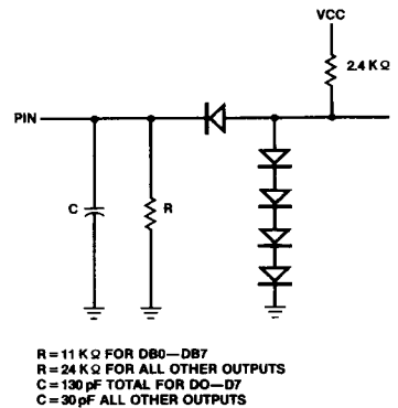
FIGURE 4. TEST LOAD
