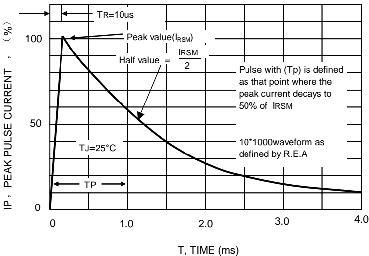
FIG.3-PULSE WAVEFORM
