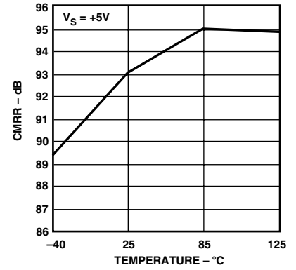
TPC 30. CMRR vs. Temperature, V_S = +5\text{ V}
