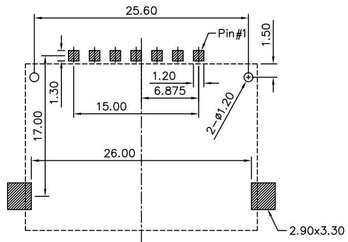
Recommended P.C.B Layout (Top View) Tolerance: ±0.10mm
