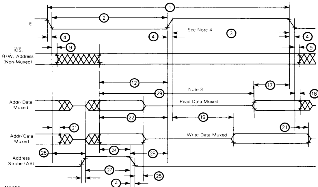
FIGURE 6 — BUS TIMING
