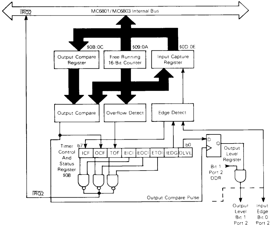
FIGURE 22 — BLOCK DIAGRAM OF PROGRAMMABLE TIMER
